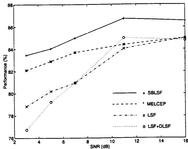
Figure 3: Performance evaluation of SBLSF, MELCEP and LSF representations.
