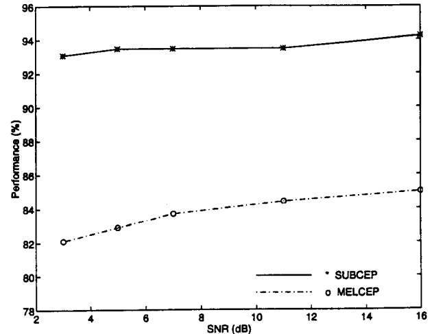
Figure 4: Performance evaluation of SUBCEP and MELCEP representations.
