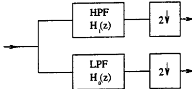
Figure 1: Basic block of subband decomposition.
