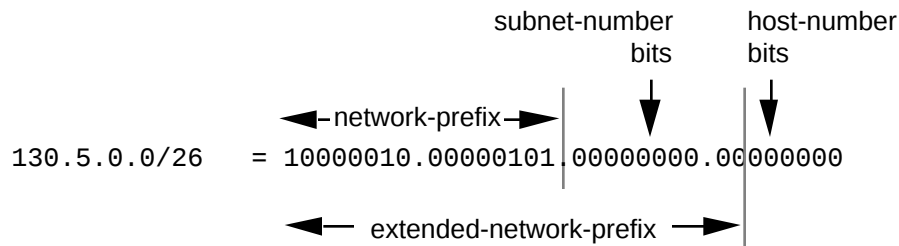
Figure 16: 130.5.0.0/16 with a /26 Extended-Network Prefix
