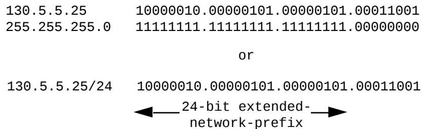
Figure 10: Extended-Network-Prefix Length
