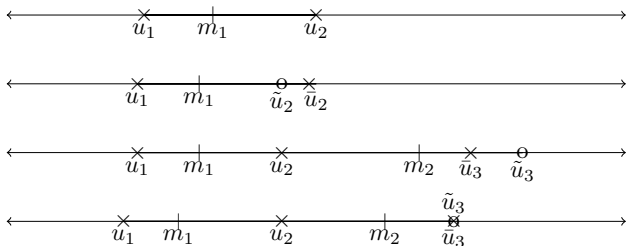
Figure 1. Illustration of the proof technique while showing the existence of equilibria with more bins when b < 0 . The first plot shows an equilibrium with two bins. In order to obtain an equilibrium with three bins, we decrease the value of bin edge m_1 . In the second plot, u_1 is the centroid of the bin (-\infty, m_1) and \tilde{u}_2 is the centroid of the bin [m_1, \infty) and \tilde{u}_2 is where the nearest neighbor condition with u_1 is satisfied at m_1 . Since \tilde{u}_2 < u_2 , we need to introduce a second bin edge m_2 so that \tilde{u}_2 is the centroid of the bin [m_1, m_2) and this is shown in the third plot. With this bin edge, we obtain a new centroid \tilde{u}_3 of the bin [m_2, \infty) . In order for this centroid to coincide with \tilde{u}_3 , we decrease m_1 further. This leads to the final plot where an equilibrium with three bins is obtained.
